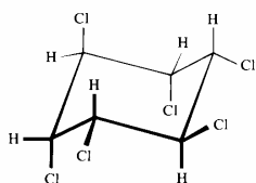
γ-1,2,3,4,5,6-Hexachlorcyclohexan (Lindan)
